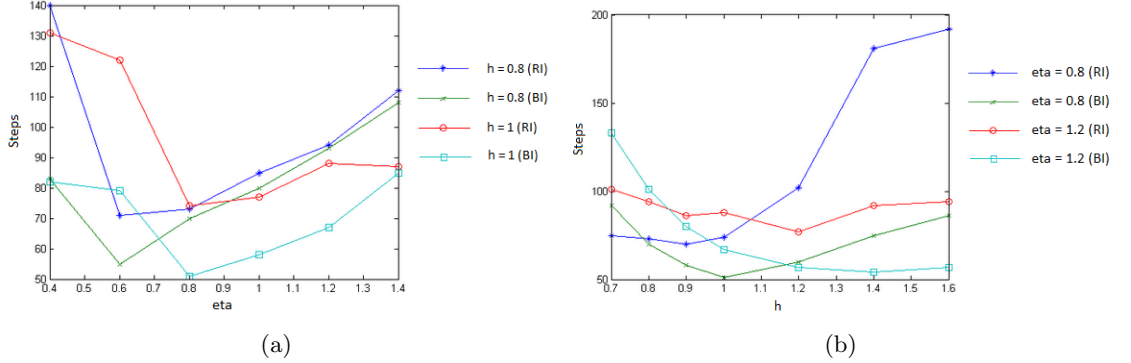
Fig. 2: Comparison between BI and RI for convergence of BP neural net with L = 3 , N(1) = 315 , N(2) = 100 , N(3) = 85 , and hyperbolic tangent activation function
