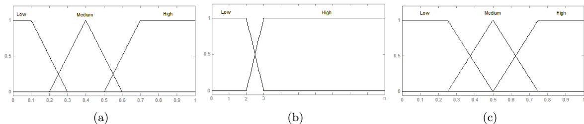
Fig. 1: Membership functions of the fuzzy sets related to, respectively, (a) d , (b) f , (c) \tilde{g} , \tilde{h} , and \rho .
